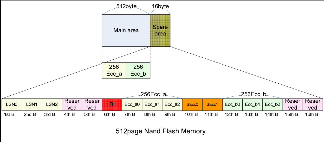
Figure 23-17 Spare area
