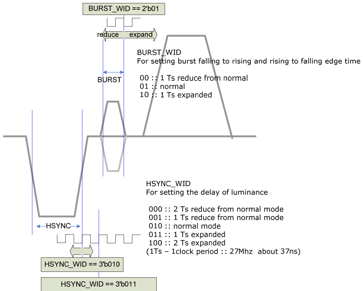
Figure 16-9 output HSYNC / BURST timing chart
