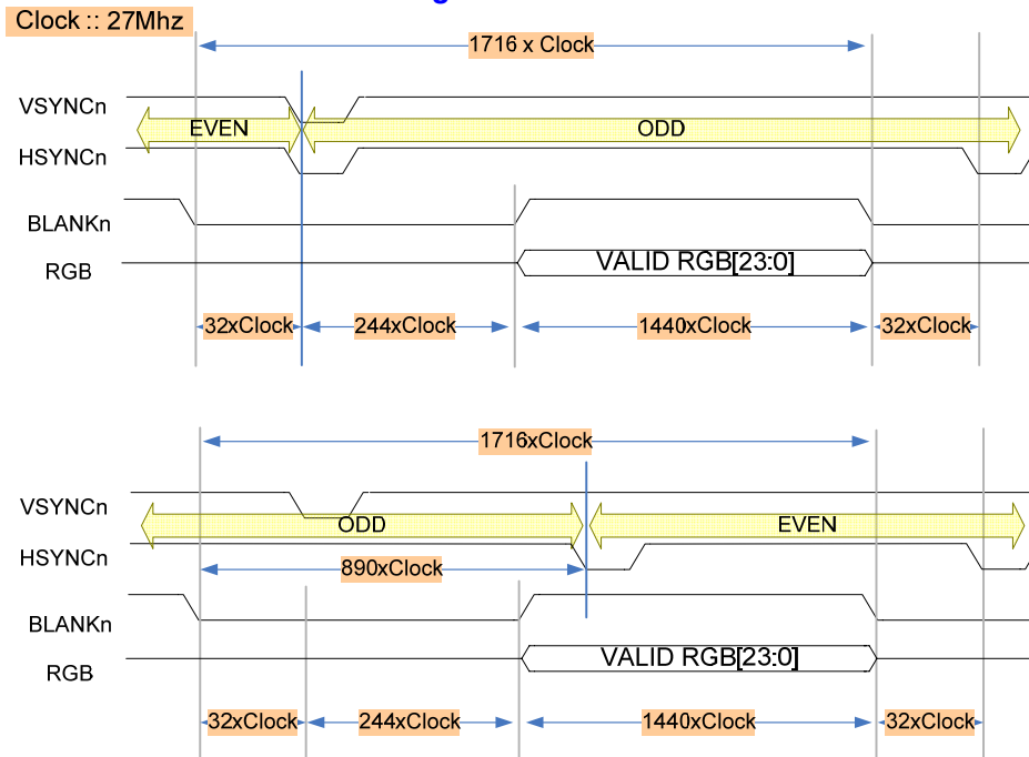
Figure 16-3 NTSC Even and Odd timing chart
