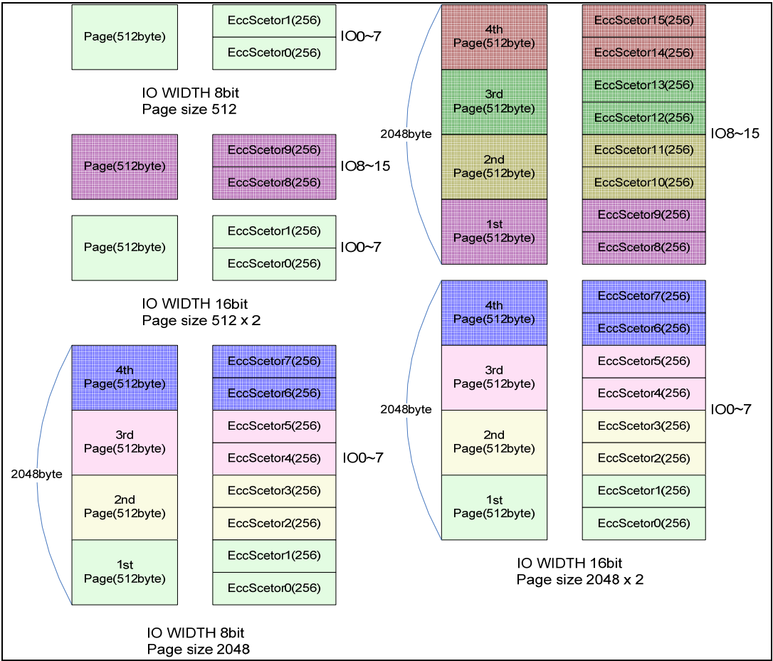
Figure 23-15 Interface별 Ecc Sector
