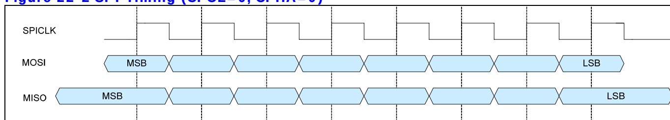
Figure 22-2 SPI Timing (CPOL=0, CPHA=0)
