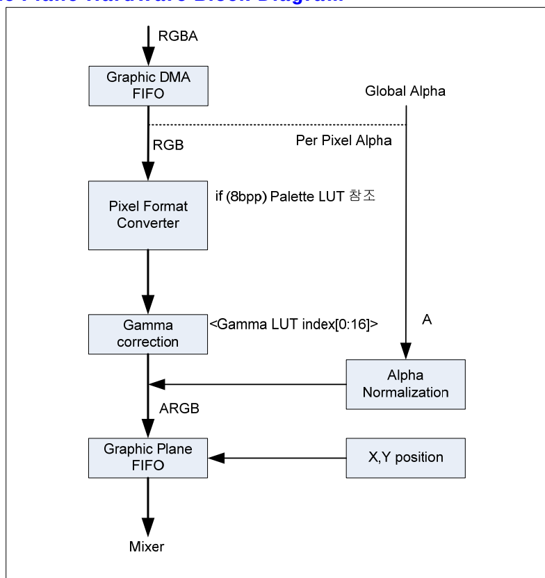
Figure 17-3 Graphic Plane Hardware Block Diagram
