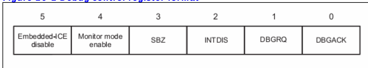
Figure 26-2 Debug control register format
