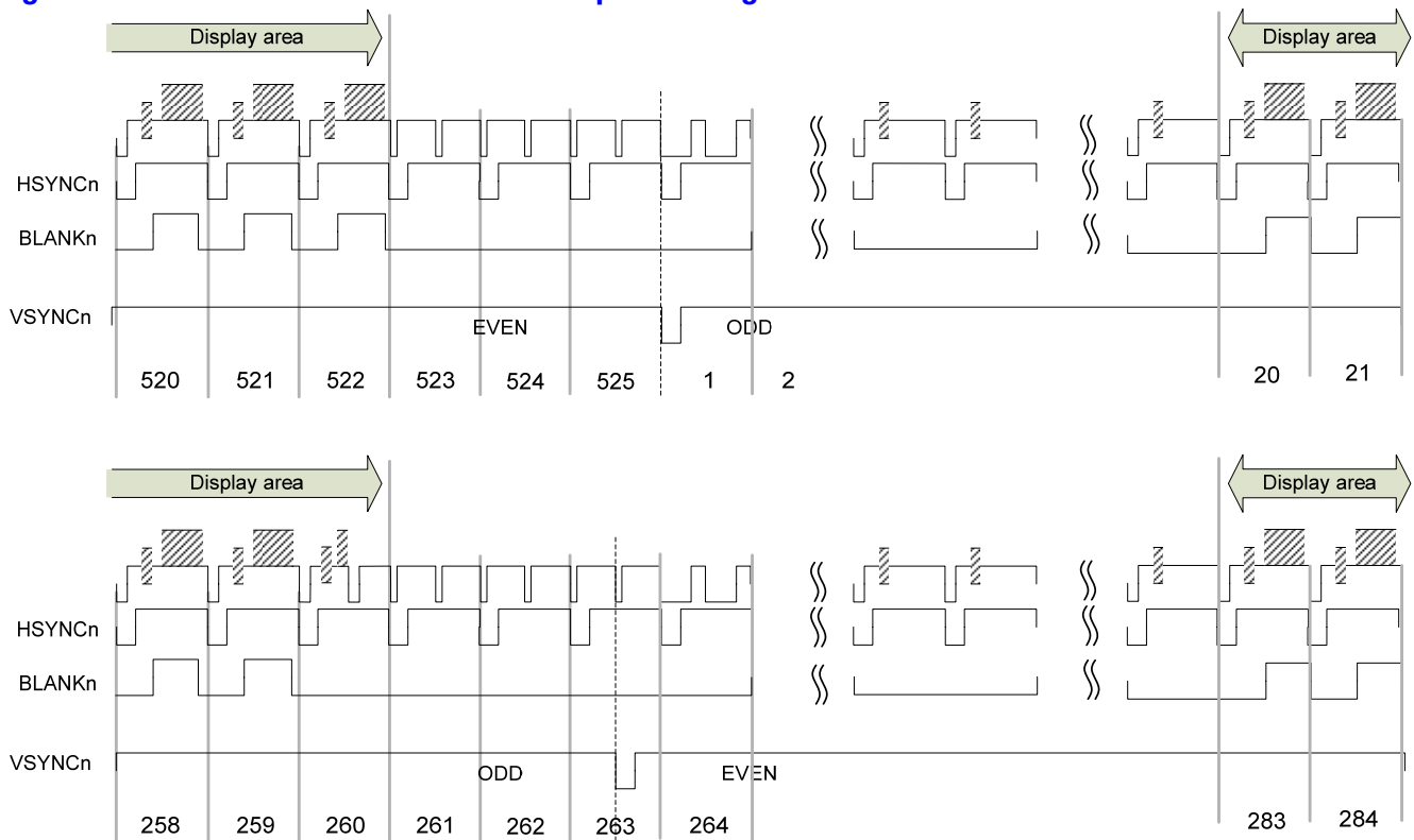
Figure 16-2 Interlaced NTSC Video input timing chart
