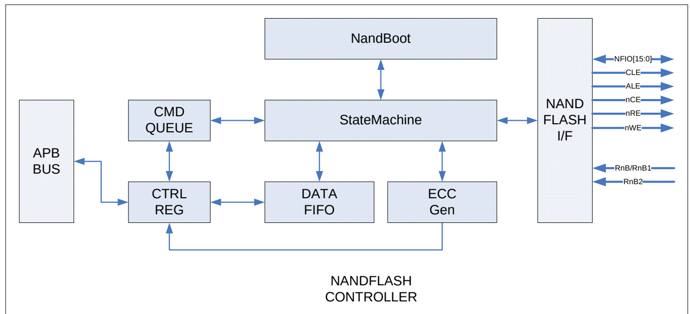
Figure 23-1 NAND Flash Controller Block Diagram
