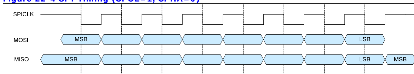
Figure 22-4 SPI Timing (CPOL=1, CPHA=0)
