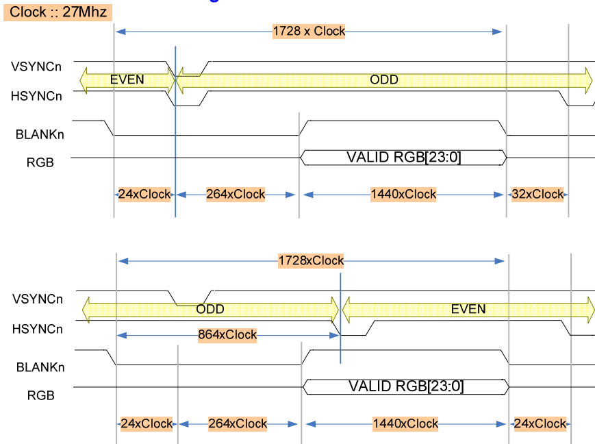
Figure 16-7 PAL Even and Odd timing chart
