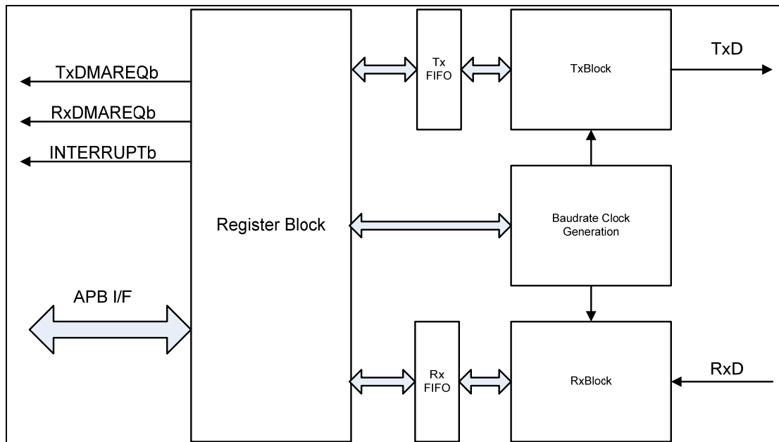
Figure 19-1 Block diagram
