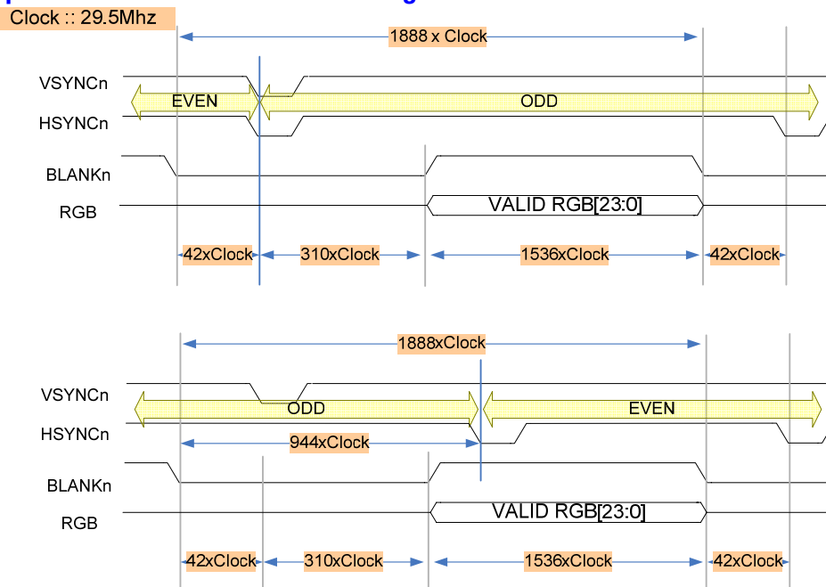
Figure 16-8 Square PAL Even and Odd timing chart
