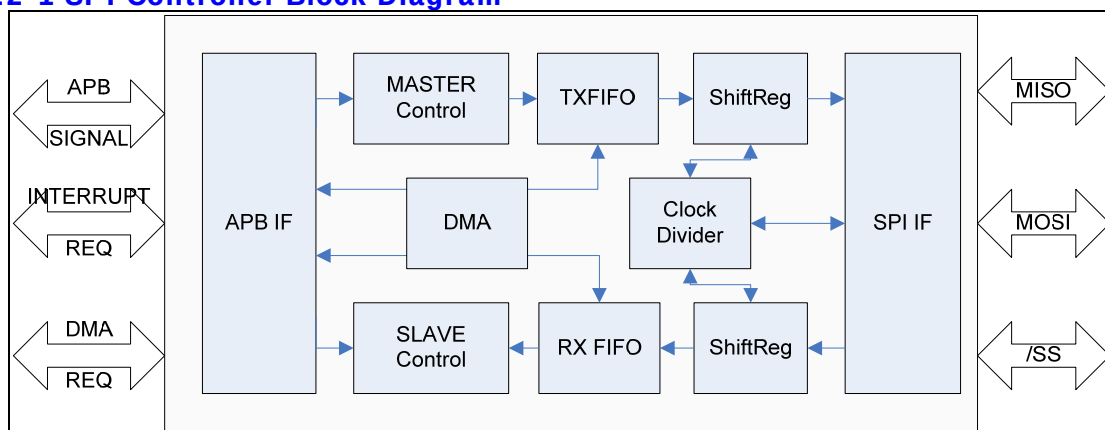
Figure 22-1 SPI Controller Block Diagram
