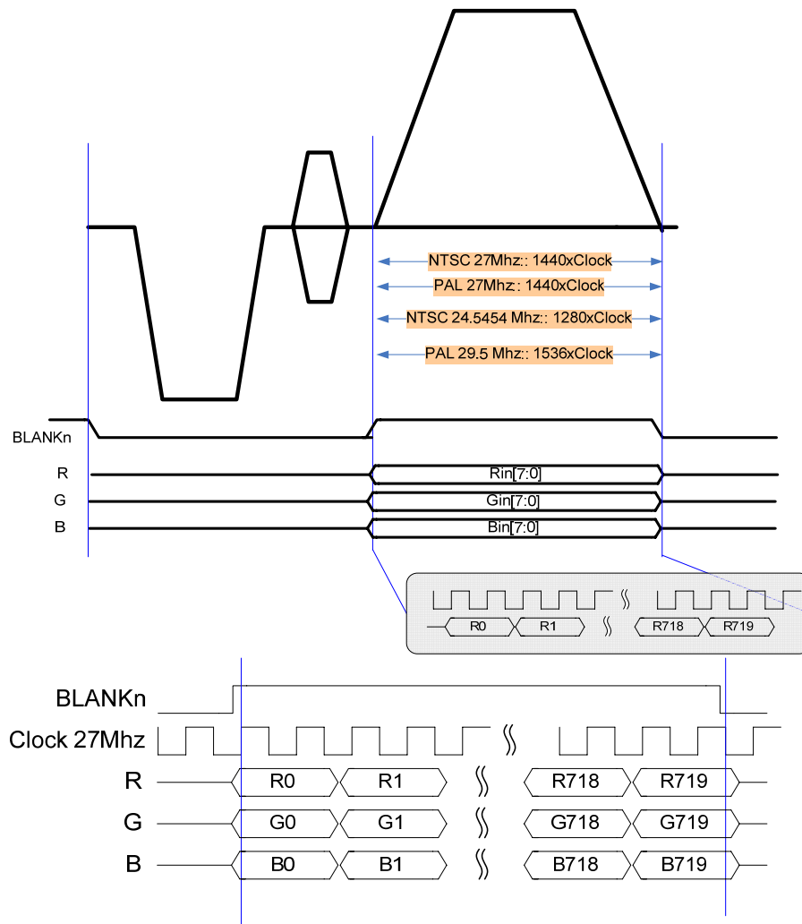
Figure 16-5 RGB input timing
