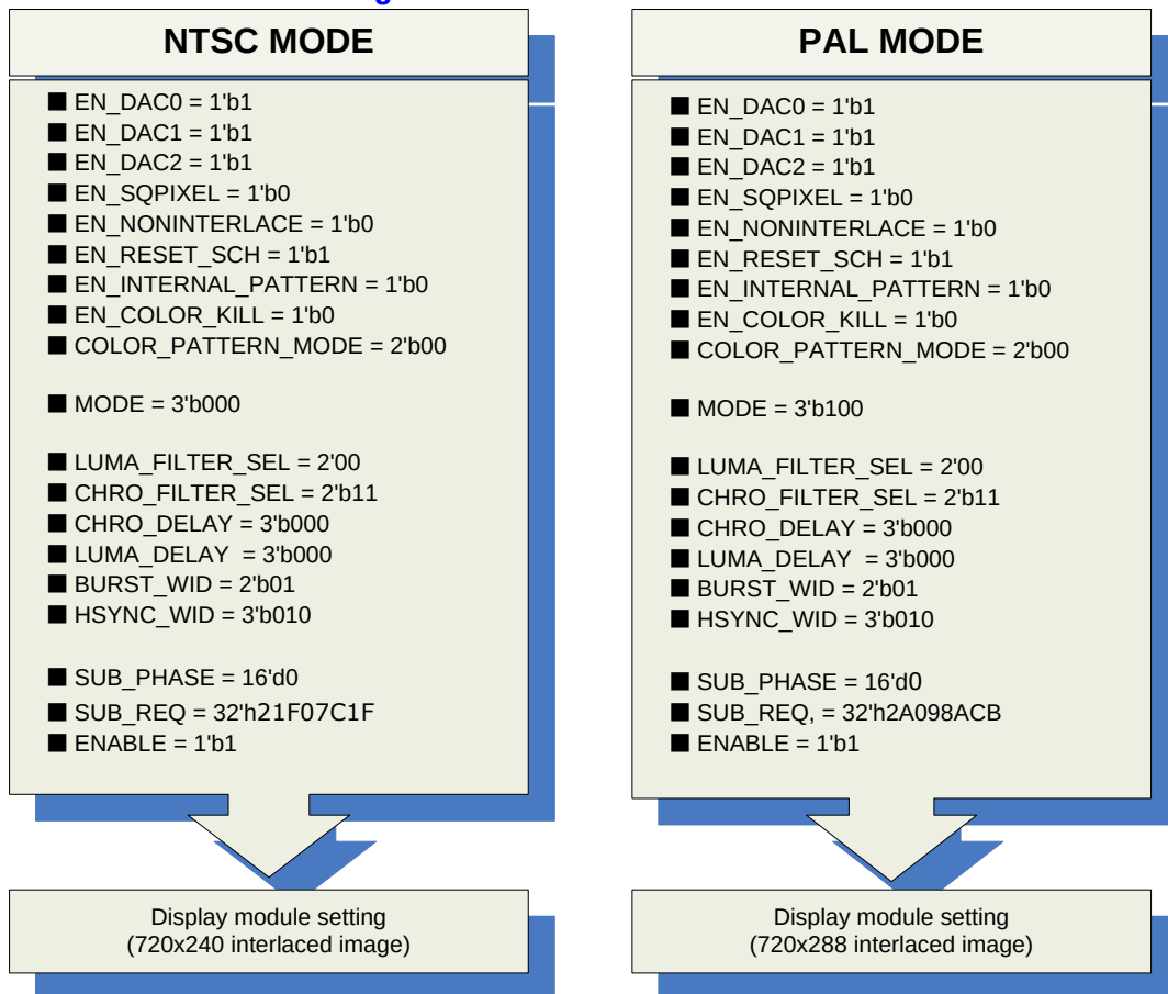
Figure 16-12 NTSC / PAL setting
