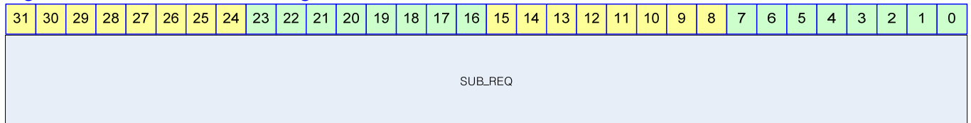
Figure 16-17 Subcarrier Register Bits
