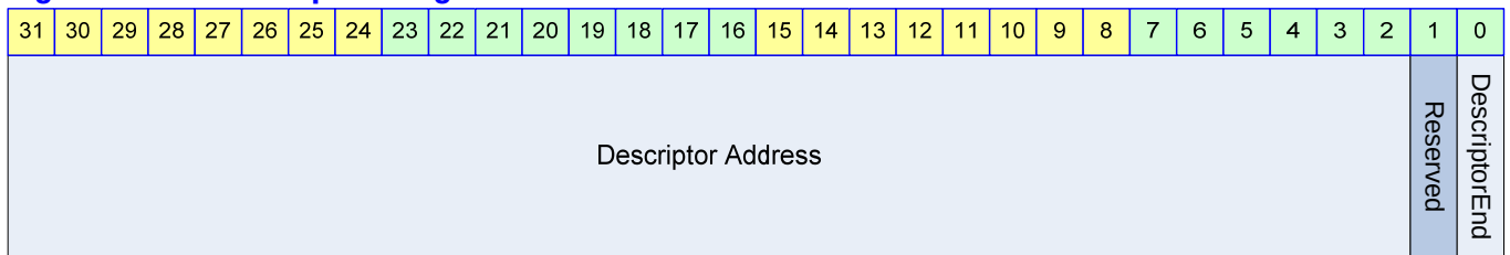
Figure 10-7 Descriptor Register
