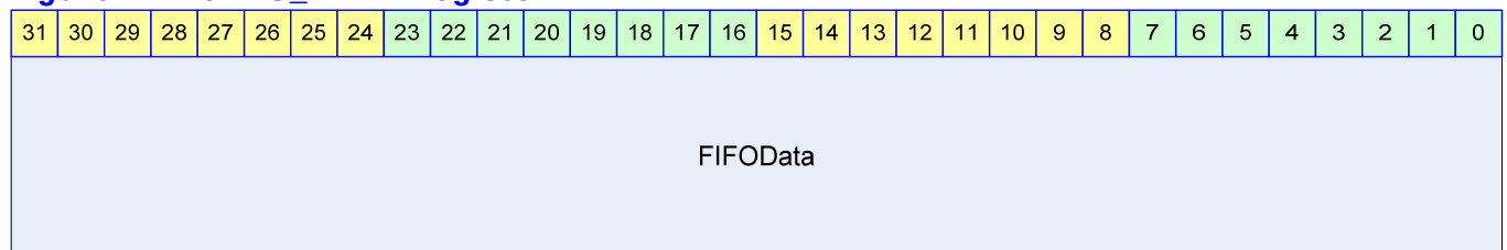
Figure 14-10 I2S_DATA Register
