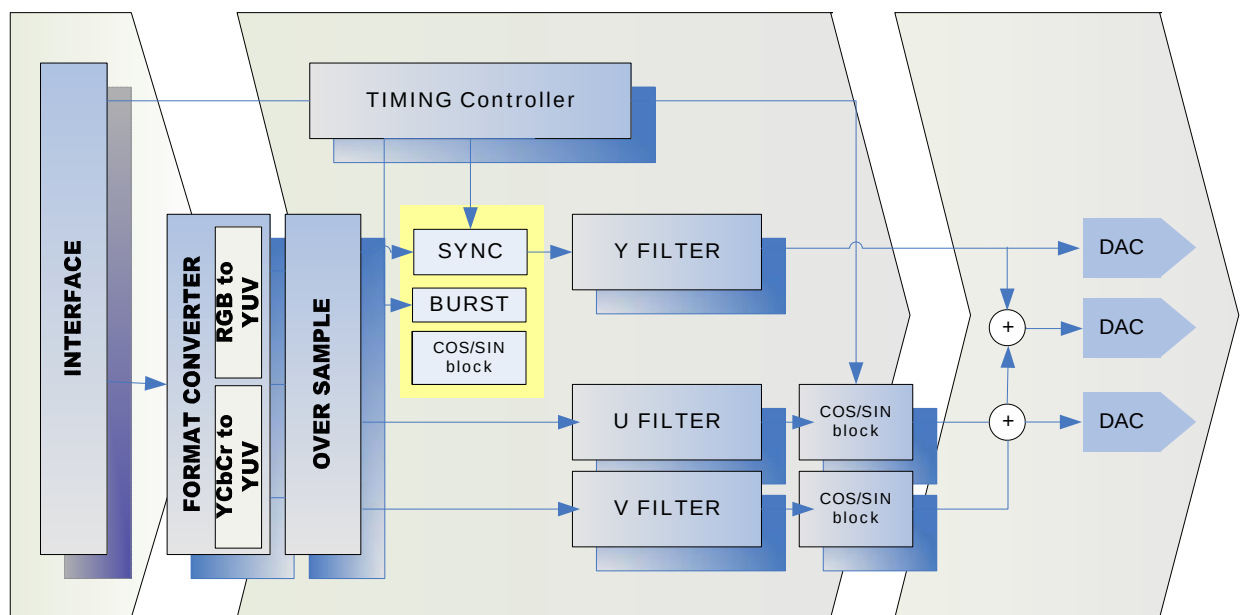
Figure 16-1 Video Encoder Block Diagram
