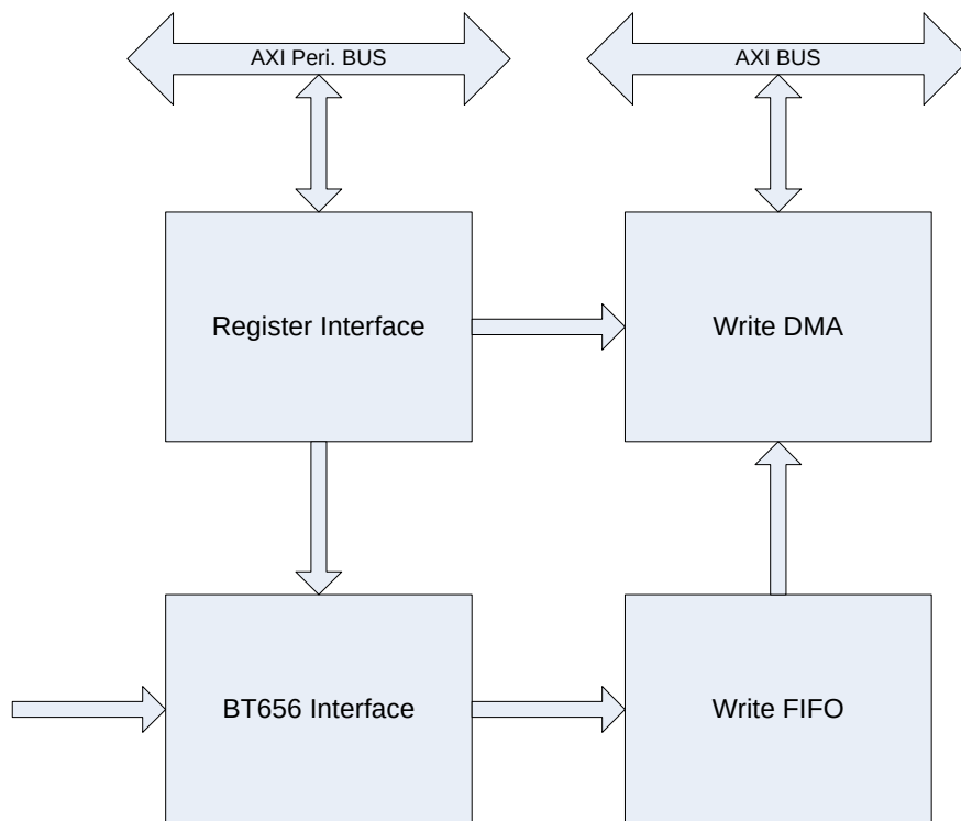
Figure 0-1 Block diagram
