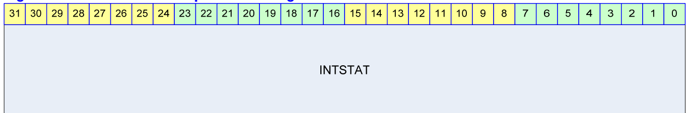
Figure 21-6 GPIO Interrupt Status Register
