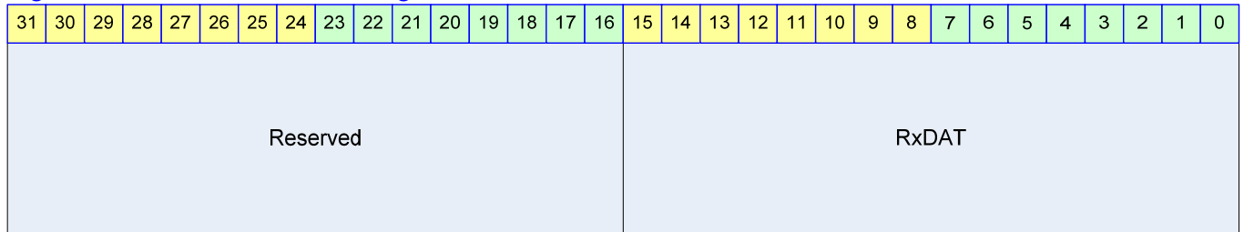
Figure 22-12 SPI Rx Data Register Bits
