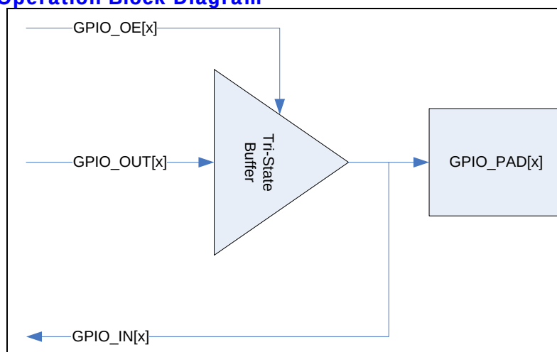
Figure 21-1 GPIO Operation Block Diagram
