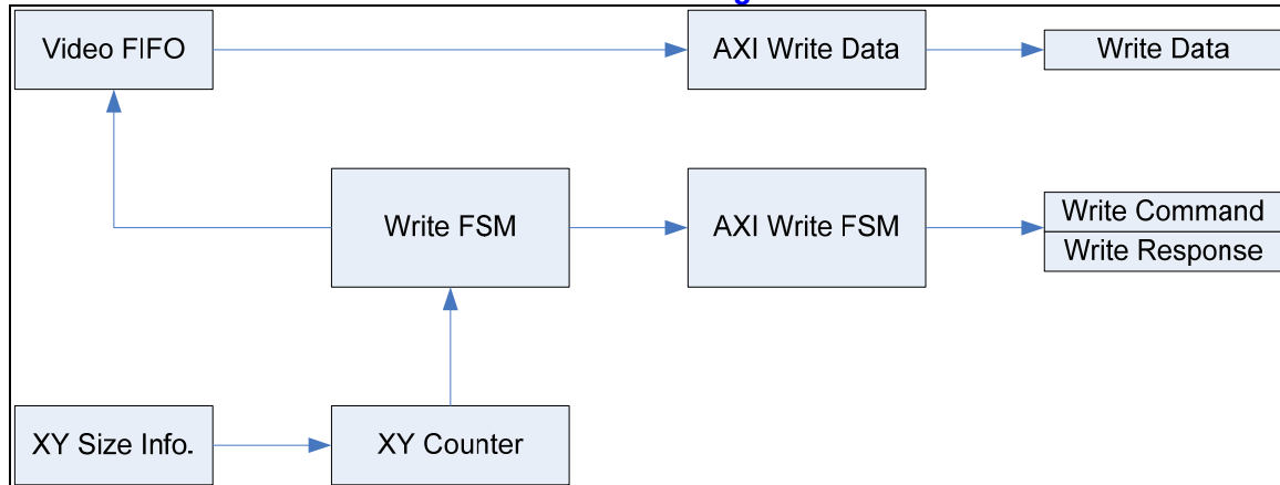
Figure 0-3 AXI BUS Write DMA Interface Block Diagram
