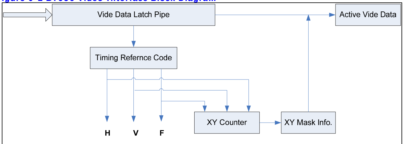
Figure 0-2 BT656 Video Interface Block Diagram
