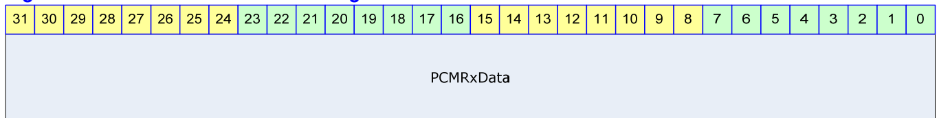
Figure 20-4 PCM RX DMA Data Register Bits
