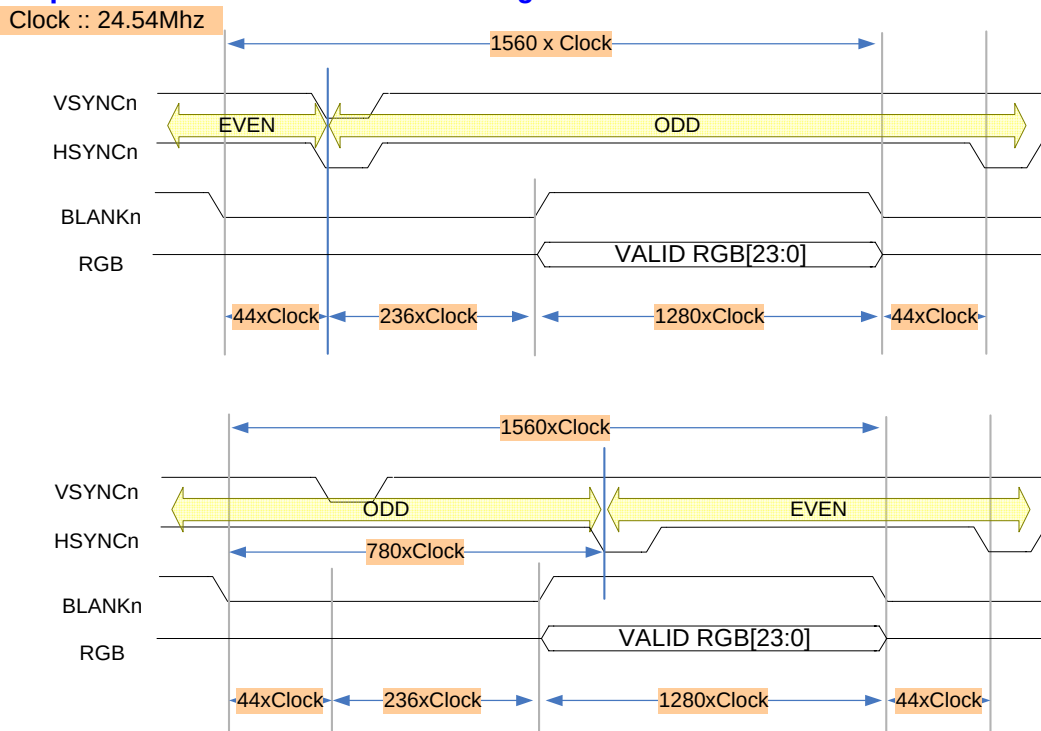
Figure 16-4 Square NTSC Even and Odd timing chart
