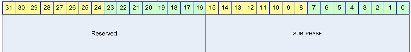
Figure 16-16 subcarrier phase Register Bits
