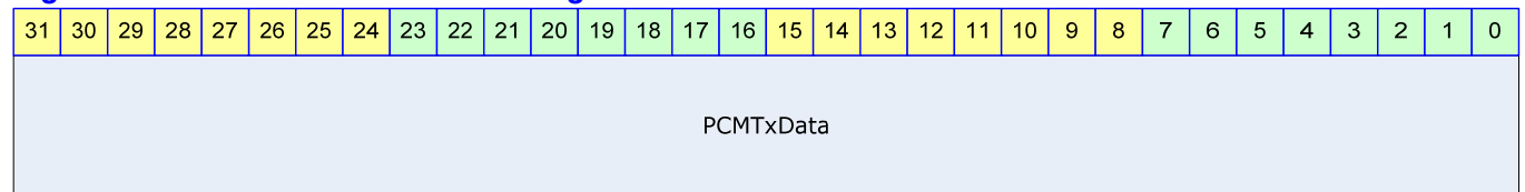
Figure 20-7 PCM TX DMA Data Register Bits
