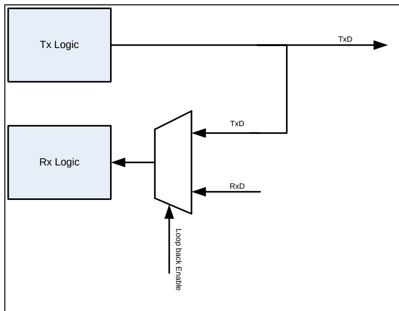
Figure 19-11 UART Loopback logic
