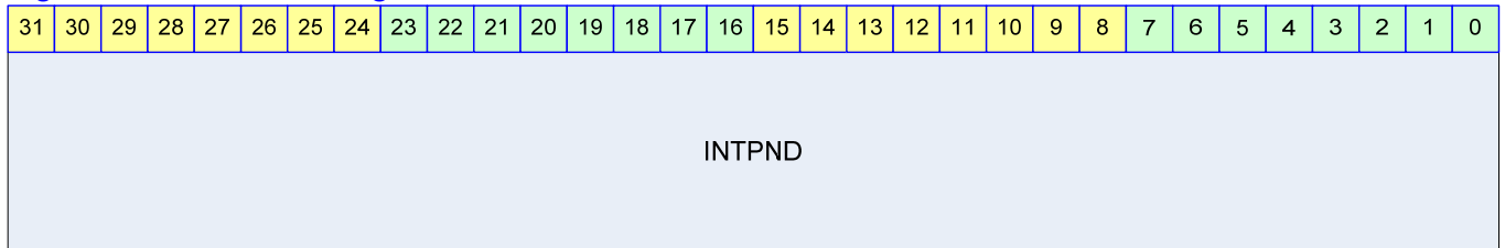
Figure 9-4 INTPND Register
