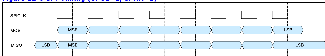
Figure 22-5 SPI Timing (CPOL=1, CPHA=1)
