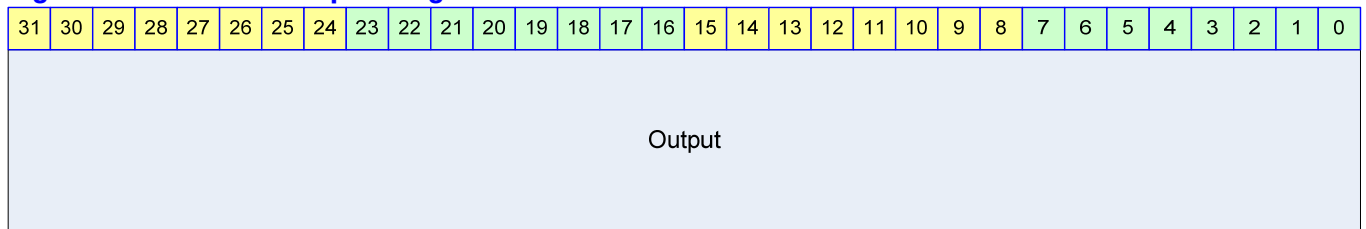
Figure 21-5 GPIO Output Register
