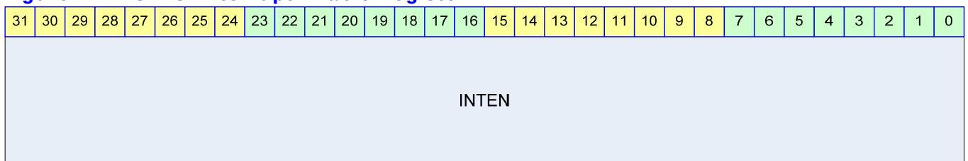
Figure 21-7 GPIO Interrupt Enable Register
