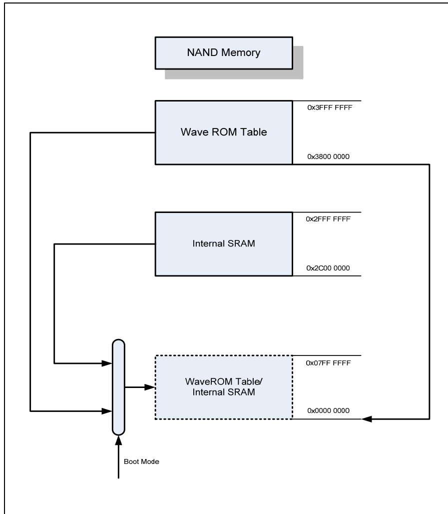
Figure 4-4 Direct boot mode
