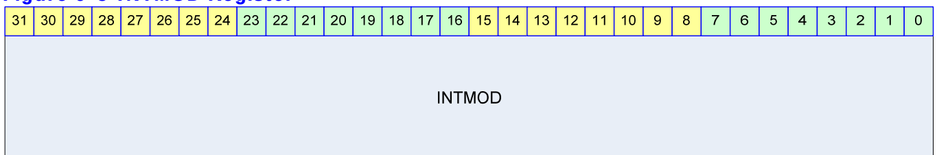
Figure 9-5 INTMOD Register
